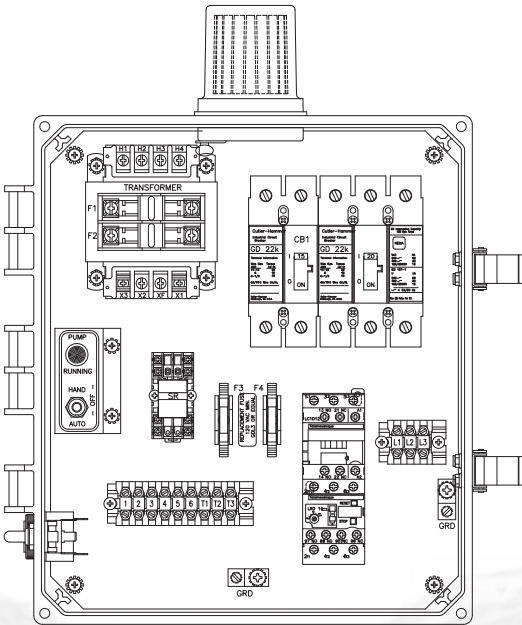
Standard Panel Layout
