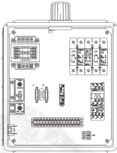
Panel Layout w/Seal Leak & Mtr Thermal OL
