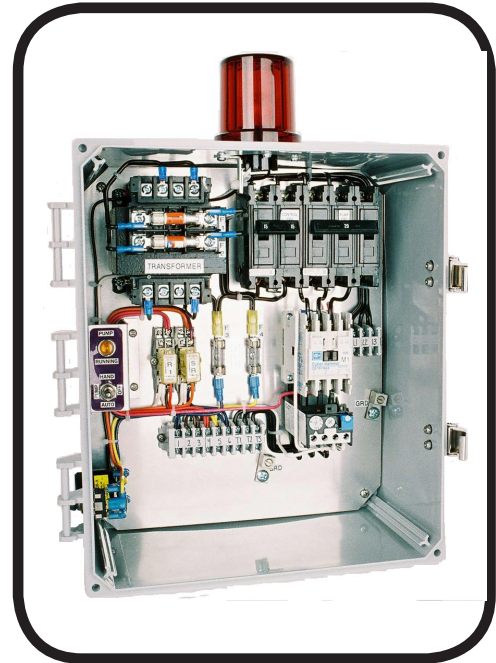
Control Panel Simplex, NEMA 4X Three Phase, 460 Volt
